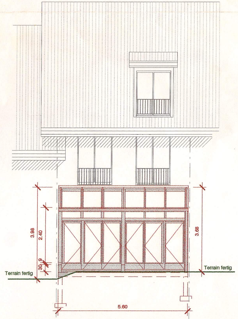
FASSADE SUED 1:100
